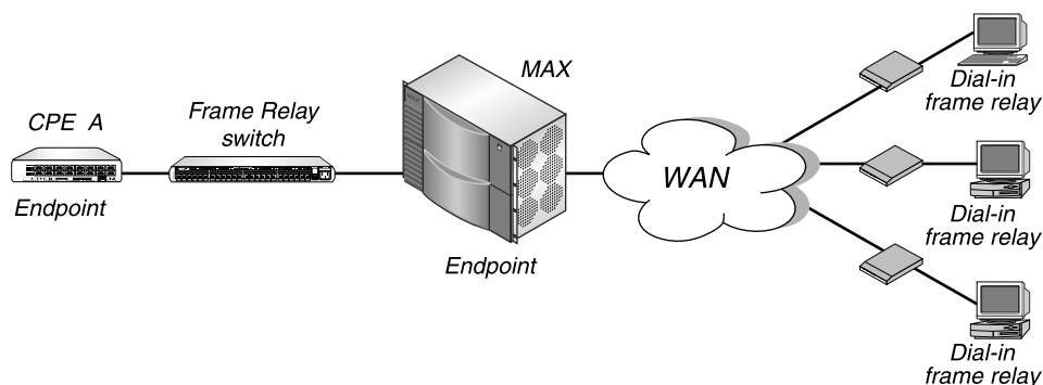
Figure 5-6. Gateway connections
