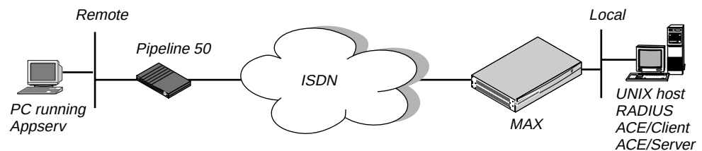
Figure 3-2 ACE/Server configuration
