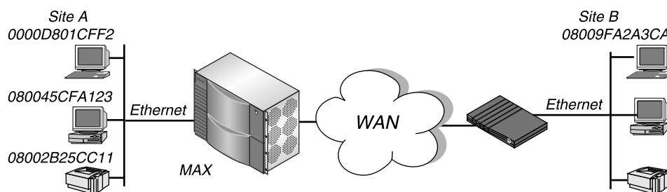
Figure 6-7 Bridging configuration
