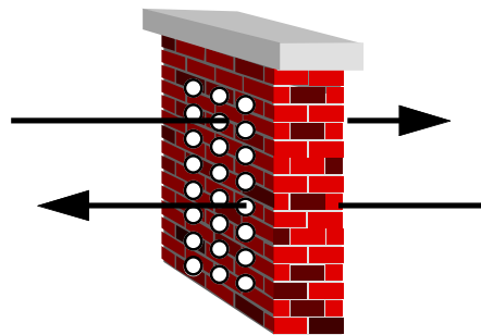
Static Filtering
