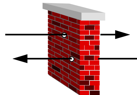
Dynamic Firewall
