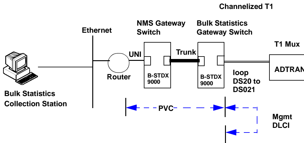
Figure 2-3. Configuration for a Large Network — Channelized T1
