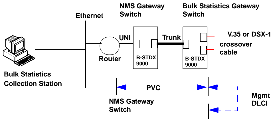
Figure 2-2. Configuration for a Large Network — V.35 or DSX-1
