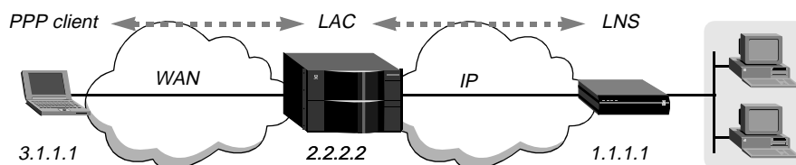
Figure 7-5. L2TP tunnel
