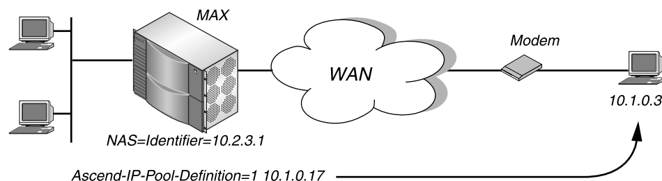
Figure 6-3. An IP routing connection with dial-in host requiring dynamic IP addressing
