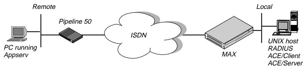
Figure 3-2. ACE/Server configuration
