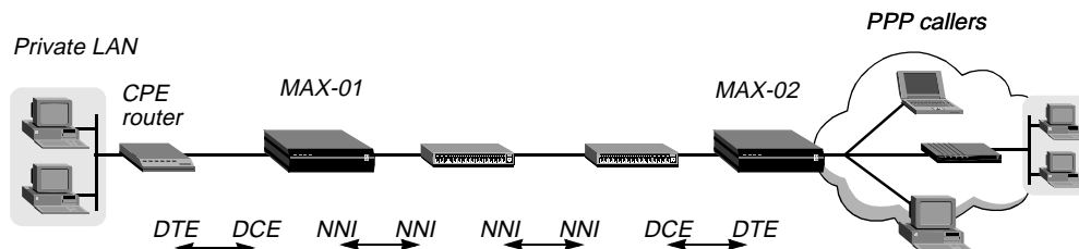
Figure 4-1. Frame Relay network
