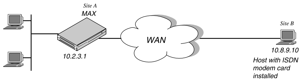
Figure 10-9. A dial-in user requiring a static IP address (a host route)
