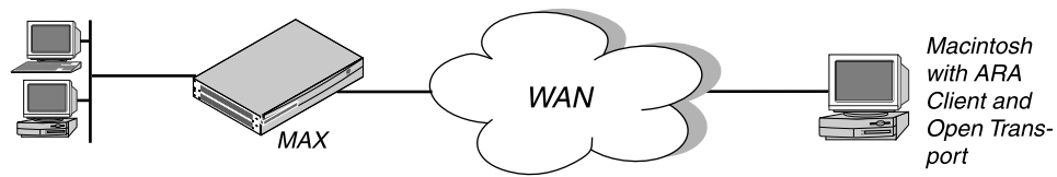
Figure 3-11. An ARA connection enabling IP access
