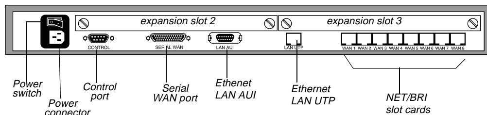
Figure 2-1. Slot and port numbering in the MAX 1800
