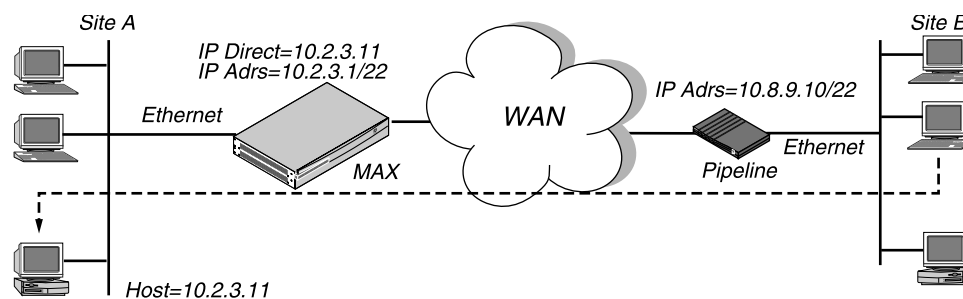
Figure 10-10. Directing incoming IP packets to one local host
