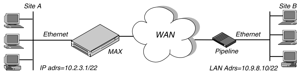
Figure 10-11. A router-to-router IP connection
