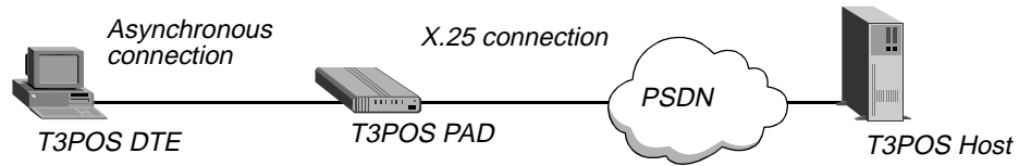
Figure 6-3. T3POS set up
