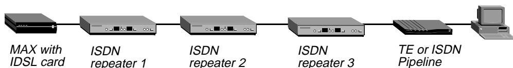
Figure 2-2. IDSL connection with repeaters
