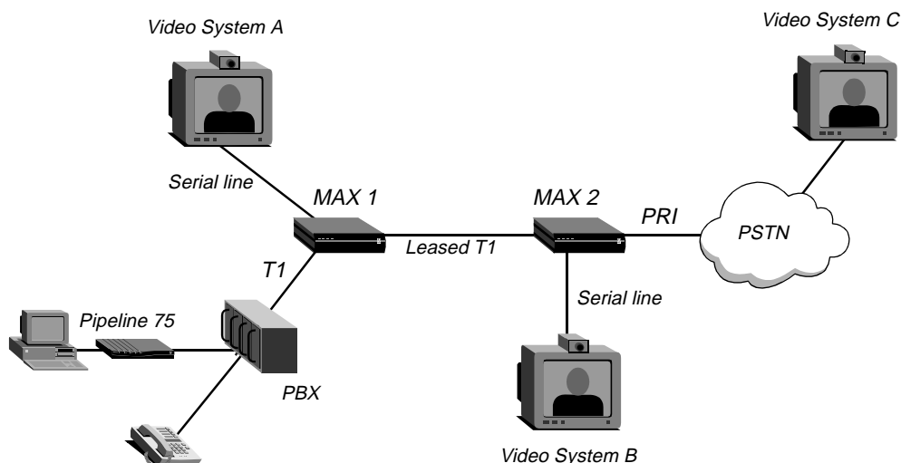
Figure 2-5. Sample MAXDAX installation
