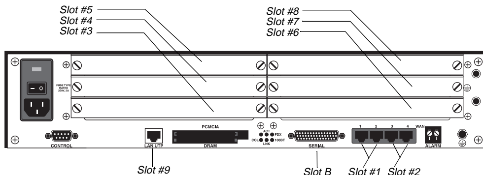
Figure 2-1. Slot and port numbering in the MAX 6000
