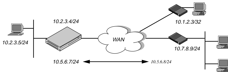
Figure 10-13. Example of a numbered interface
