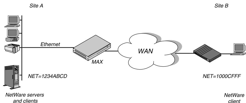
Figure 9-3. A dial-in client that belongs to its own IPX network
