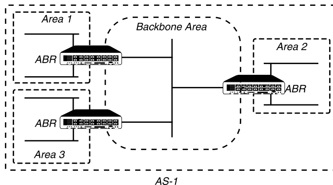
Figure 11-5. Dividing an AS into areas
