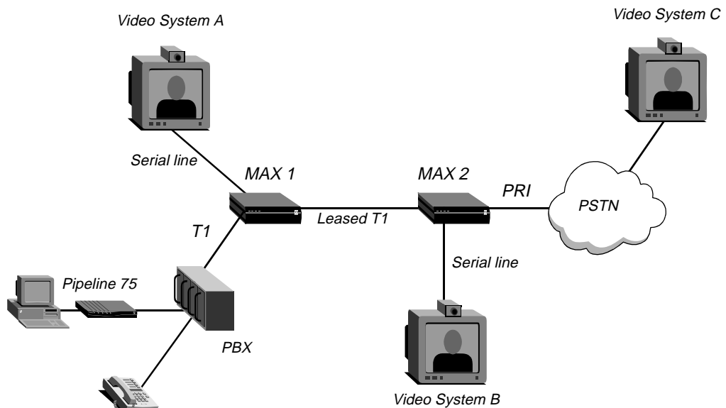
Figure 2-3. Sample MAXDAX environment
