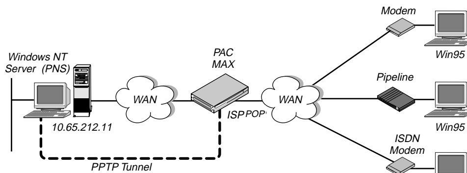
Figure 13-6. PPTP tunnel
