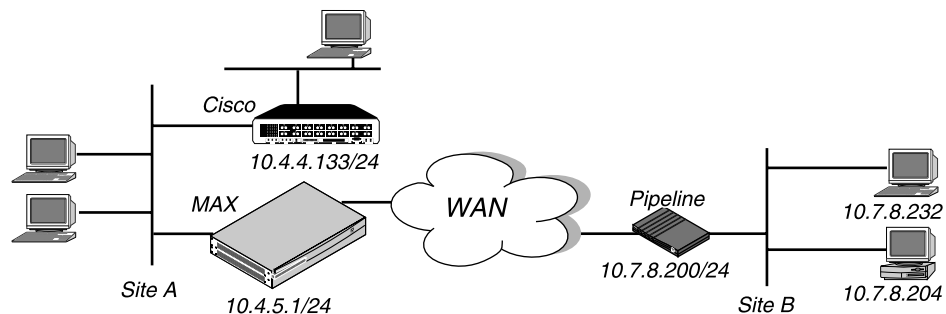
Figure 10-12. A connection between local and remote subnets
