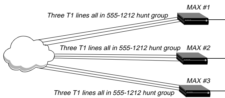
Figure 3-8. Hunt groups for a MAX stack handling only MP-without-BACP calls
