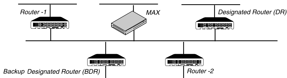
Figure 11-3. Designated and backup designated routers
